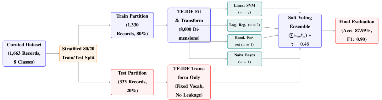
Figure 14: System Design Training, Validation, and Partitioning Workflow
